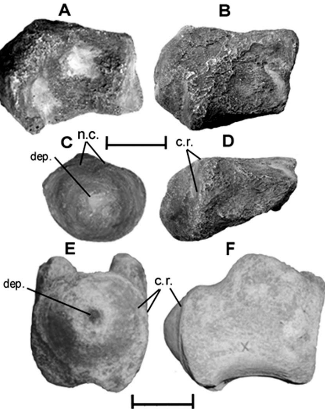
Fig.2. The fossil titanosaurian caudal centrum (CD.586) from Mangahouanga Stream (A-D) compared with an unidentified titanosaurian caudal (MACN unnumbered) from Argentina (E-F). (A) Ventral view, showing two cavities (light regions) in the centrum; (B) dorsal view; (C) posterior view; (D) right lateral view; (E) posterior view; (F) left lateral view, reversed for comparison. The conical forms of the condyles can be seen in outline in A, B, D, and F. The depression at the apex of the condyle of CD.586 retains some matrix and hence is light in color, but that of the MACN caudal is dark from shadow. The photos are of a cast of the specimen. Abbreviations: (c.r.) circumferential rim; (dep.) apical depression; (n.c.) base of neural canal. Scale bars = 50mm.
